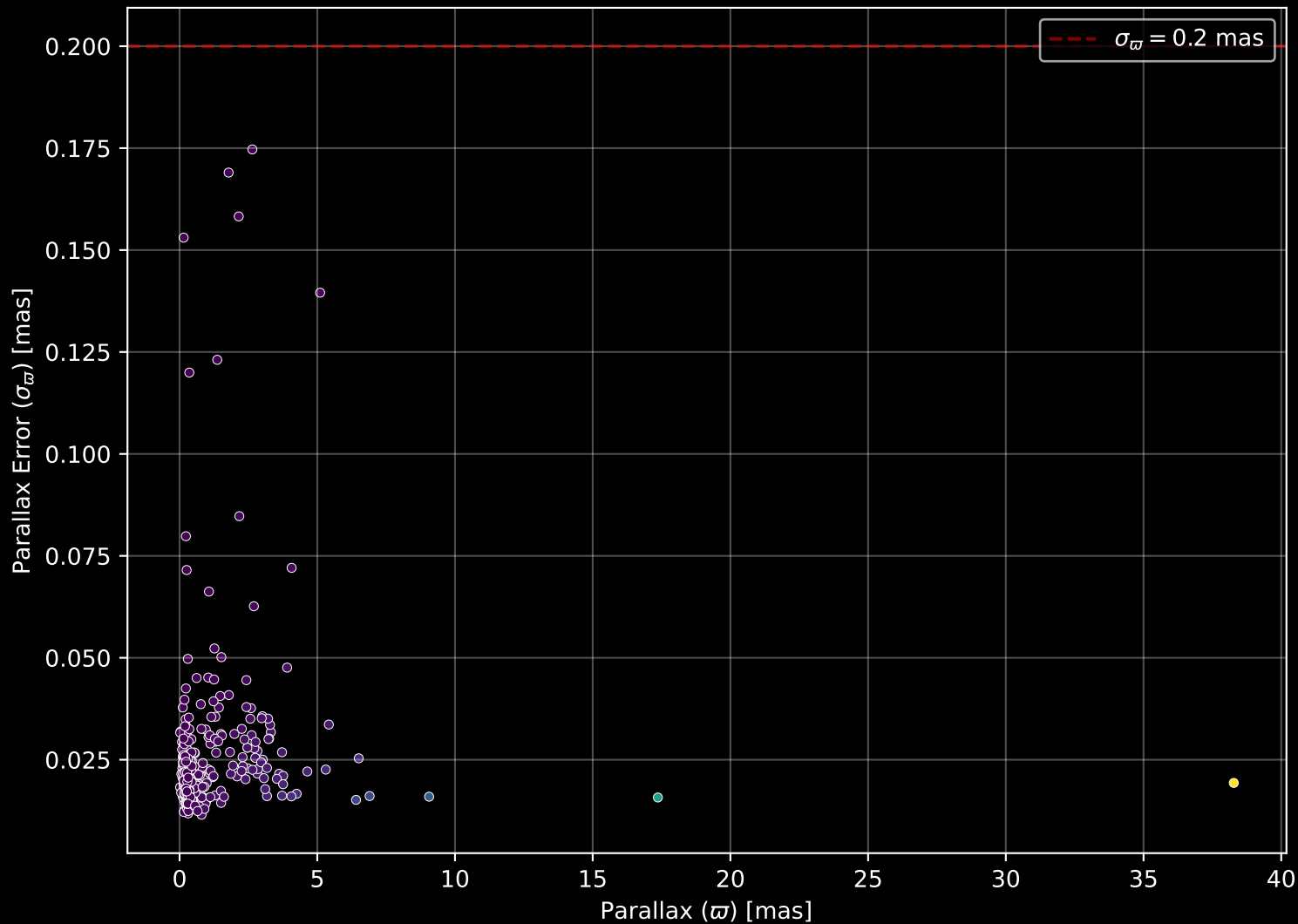
APOGEE DR17 Field: [195+08] Parallax Quality (n= 445)
