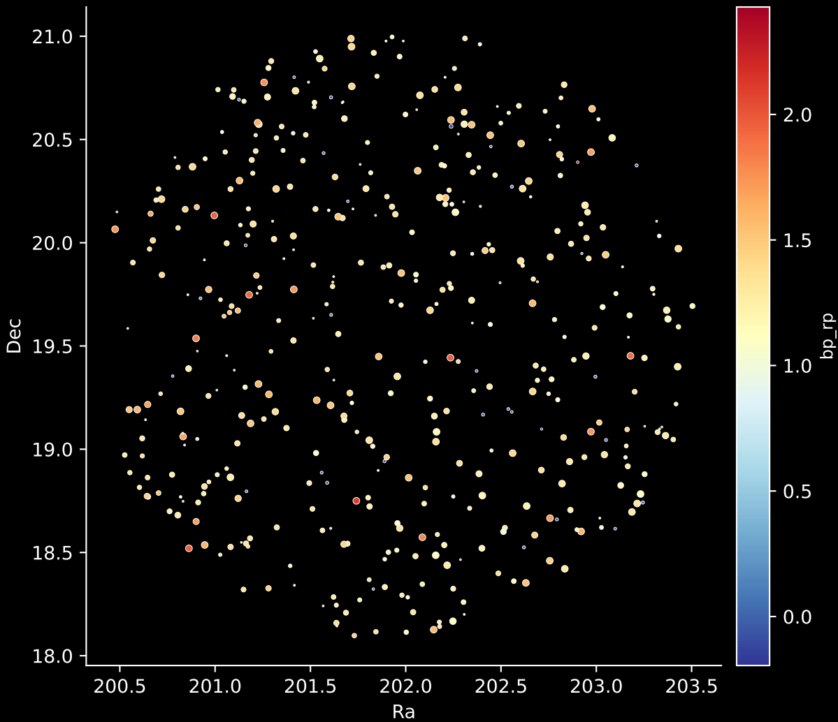
APOGEE DR17 Field: [195+08] Stars: 445
