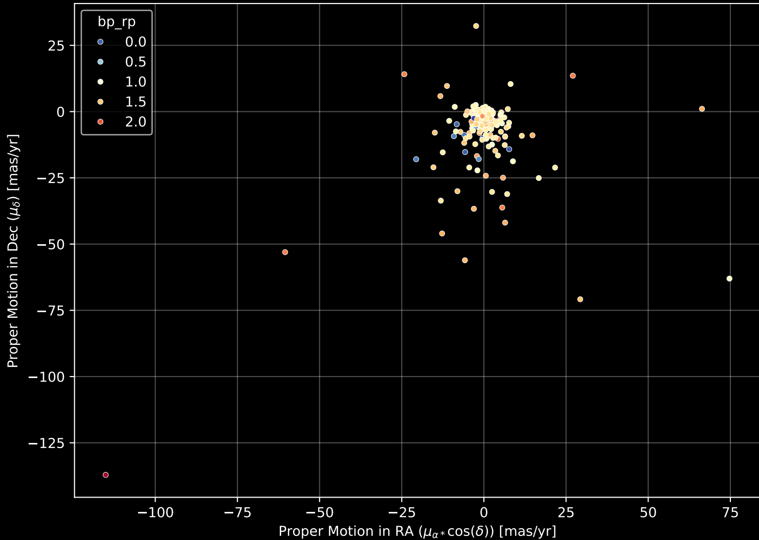
APOGEE DR17 Field: [195+08] Proper Motion Diagram (n= 445)
