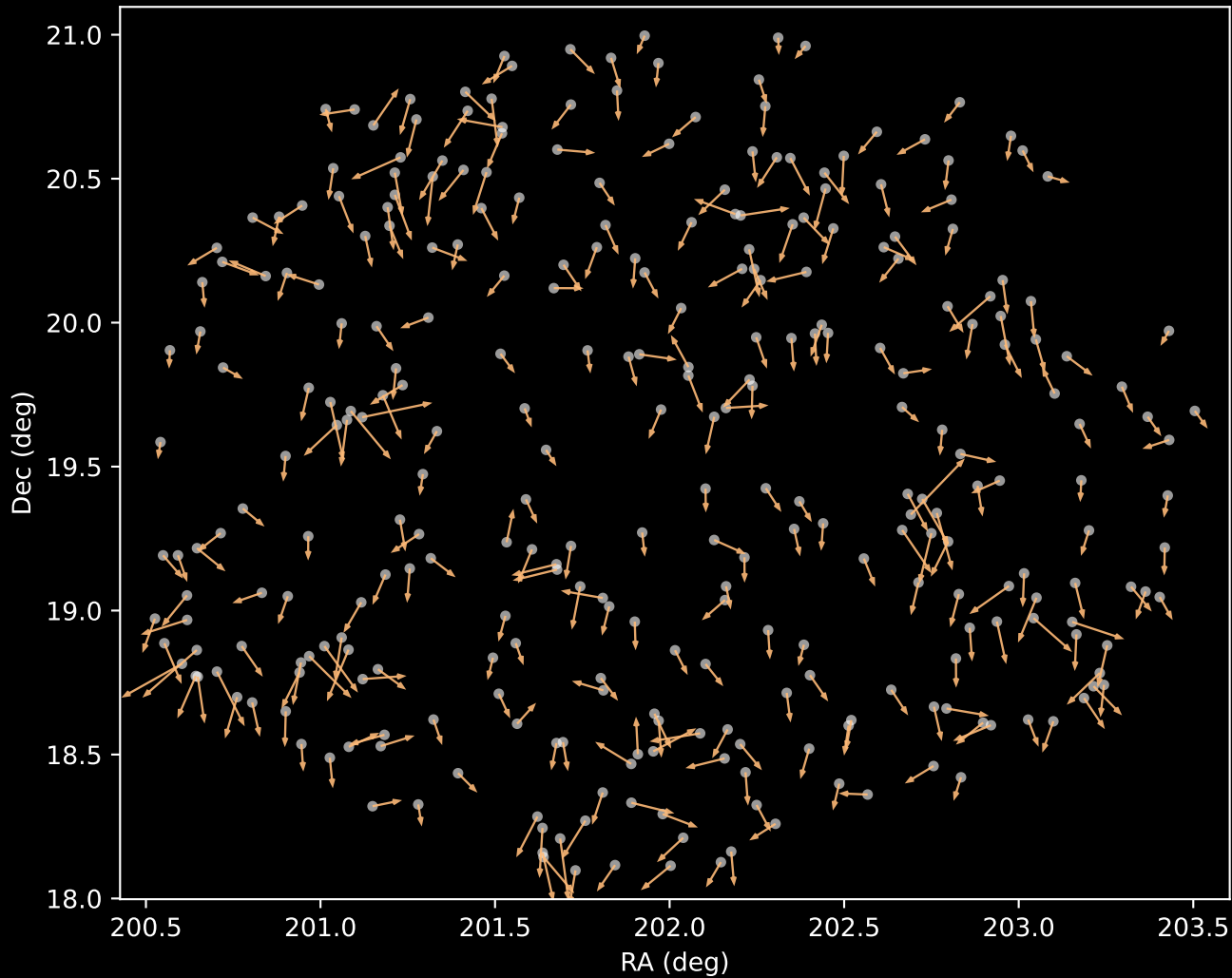
APOGEE DR17 Cluster 3 Proper Motion Vectors (n=302)
