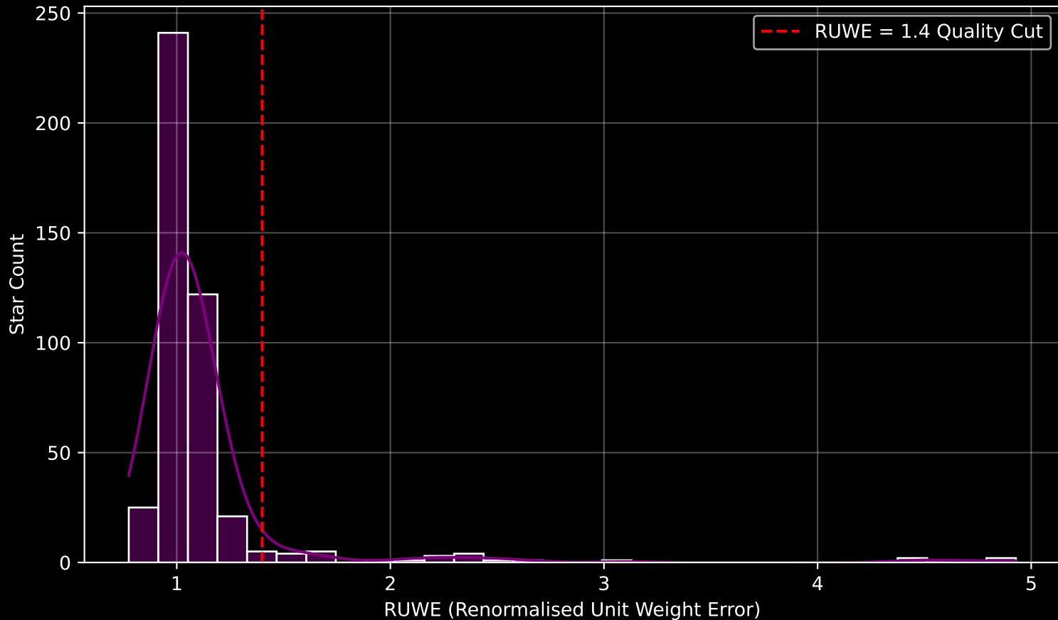
GAPOGEE DR17 Field [195+08] RUWE Distribution (n= 440)
