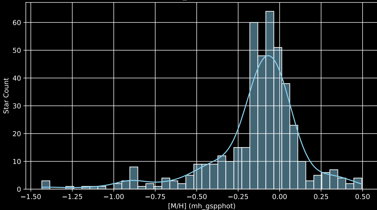
APOGEE DR17 Field: [195+08 [M/H] (mh_gspphot) (n= 442)
